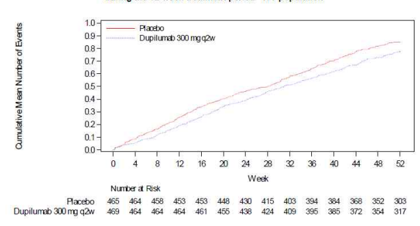
Figure 24 - Plot of cumulative mean number of COPD exacerbation events assessed by EXACT during the 52-week treatment period - ITT population
